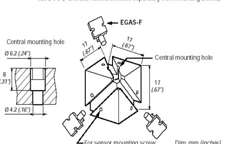
MTG-F3 (Purchase Accelerometers separately from mounting blocks)
