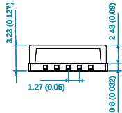
VS9000 side view
